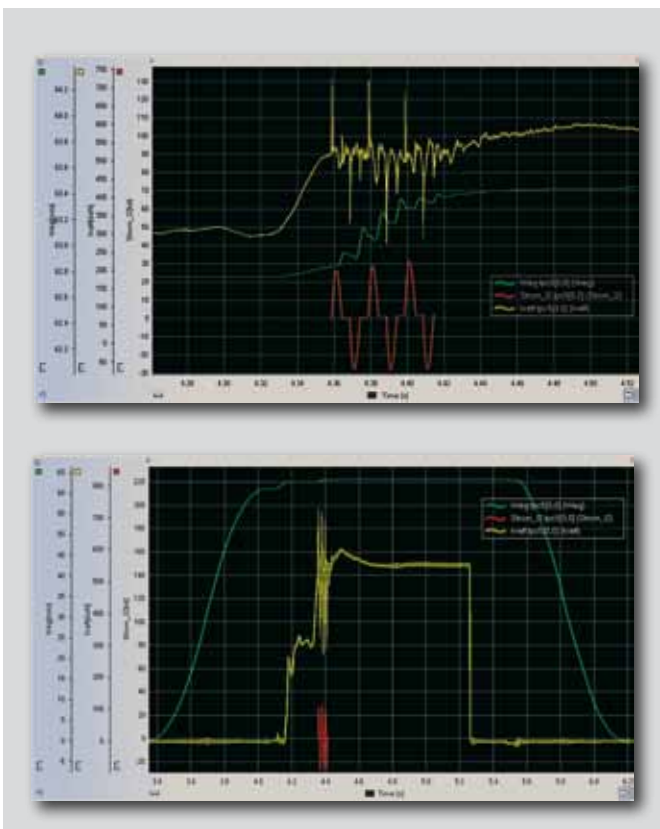
SCHEMATIC: DYNAMIC CHARACTERISTICS OF A SERVO-MOTOR DALEX-PROJECTION WELDING MACHINE WITH SERVOTRONIC®
