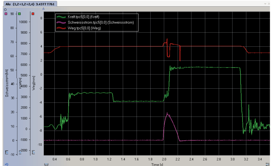
pict. weld chart current-force-movement of DALEX-Sprinter HP cylinder
